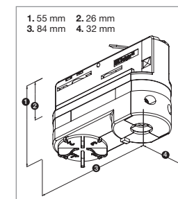
10A Multi-circuit adapter Connection with screw
